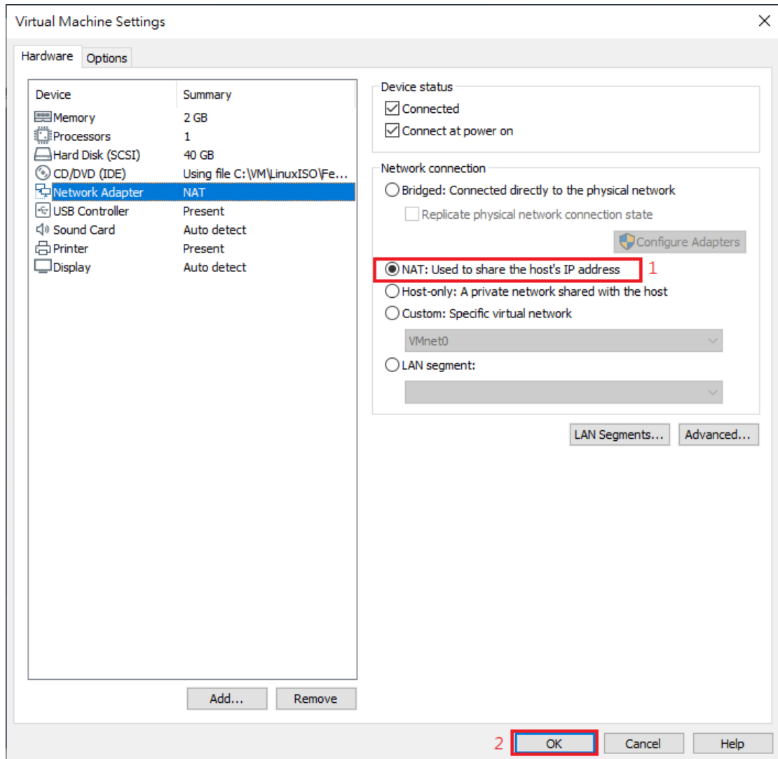
Figure21 點選 Network Adapter “NAT”
