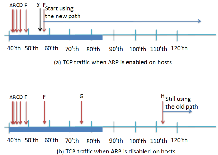
Fig. 3: The timeline for a TCP flow to change/keep its path after the link between nodes 6 and 7 breaks at 40'th sec while using NOX
